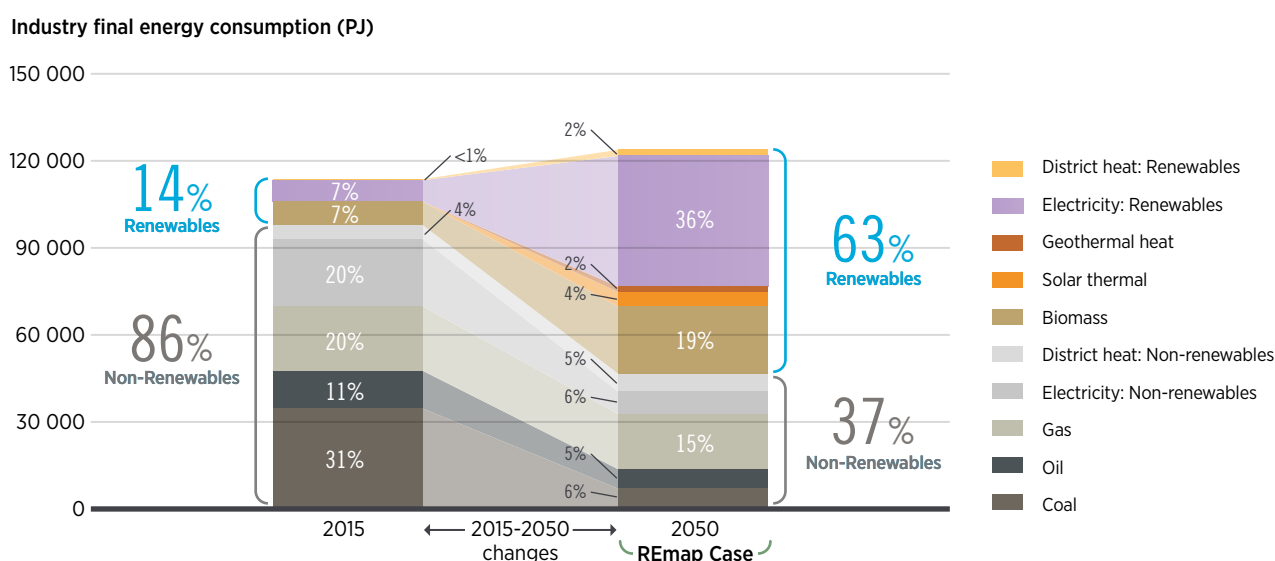
Figure 13. A diverse energy mix with sizeable bioenergy demand
